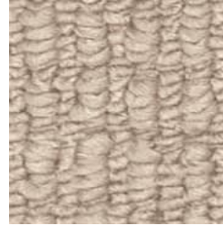
13 Waterspout
