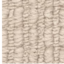
11 Wind Shear
