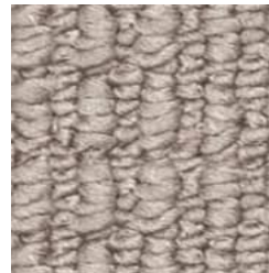
92 Dust Storm
